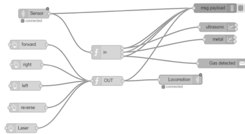
Figure 8. Broker Program
