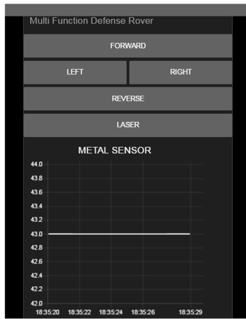
Figure 7. User Interface
